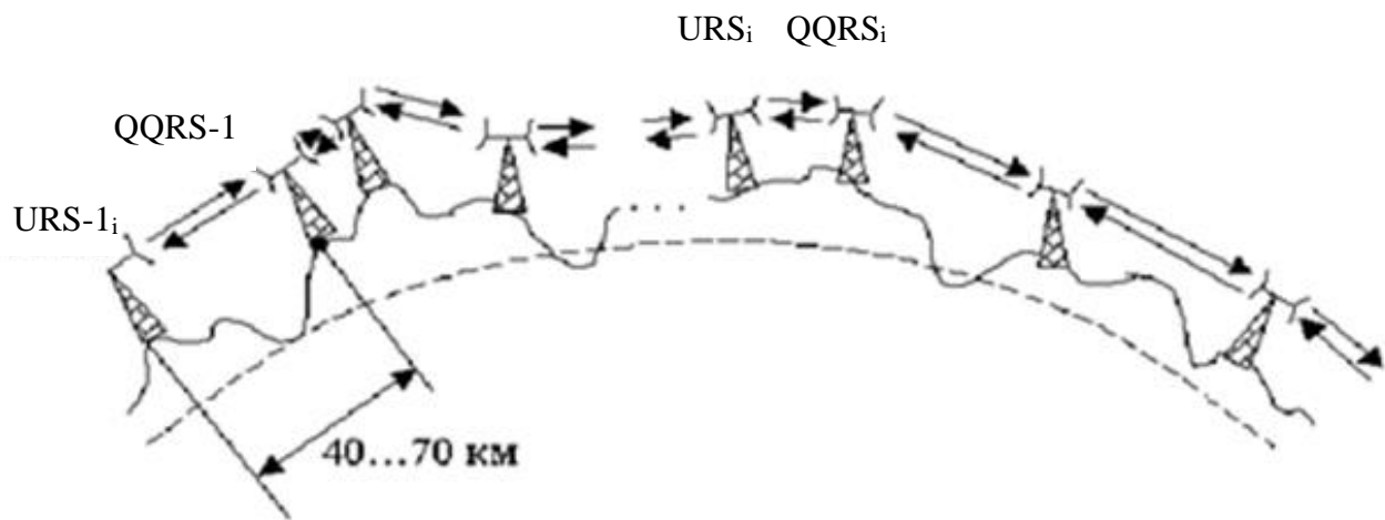
4.1-rasm. Aloqaning radioreleyli liniyasining struktura sxemasi (AXM - axborot manbai, AP - axborot priemnigi, Per - peredatchik, Pr - priyomnik)
