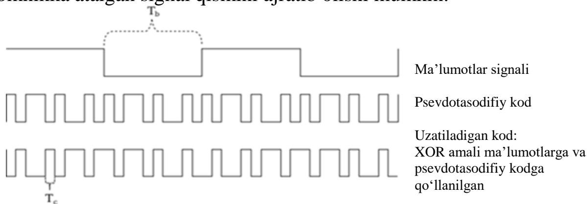
1.11-rasm. CDMA signalining generatsiyasi
