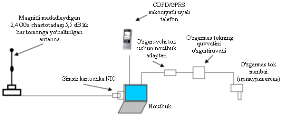
5.7-rasm. "Simsiz urushni" olib borish asbob-uskunasi
