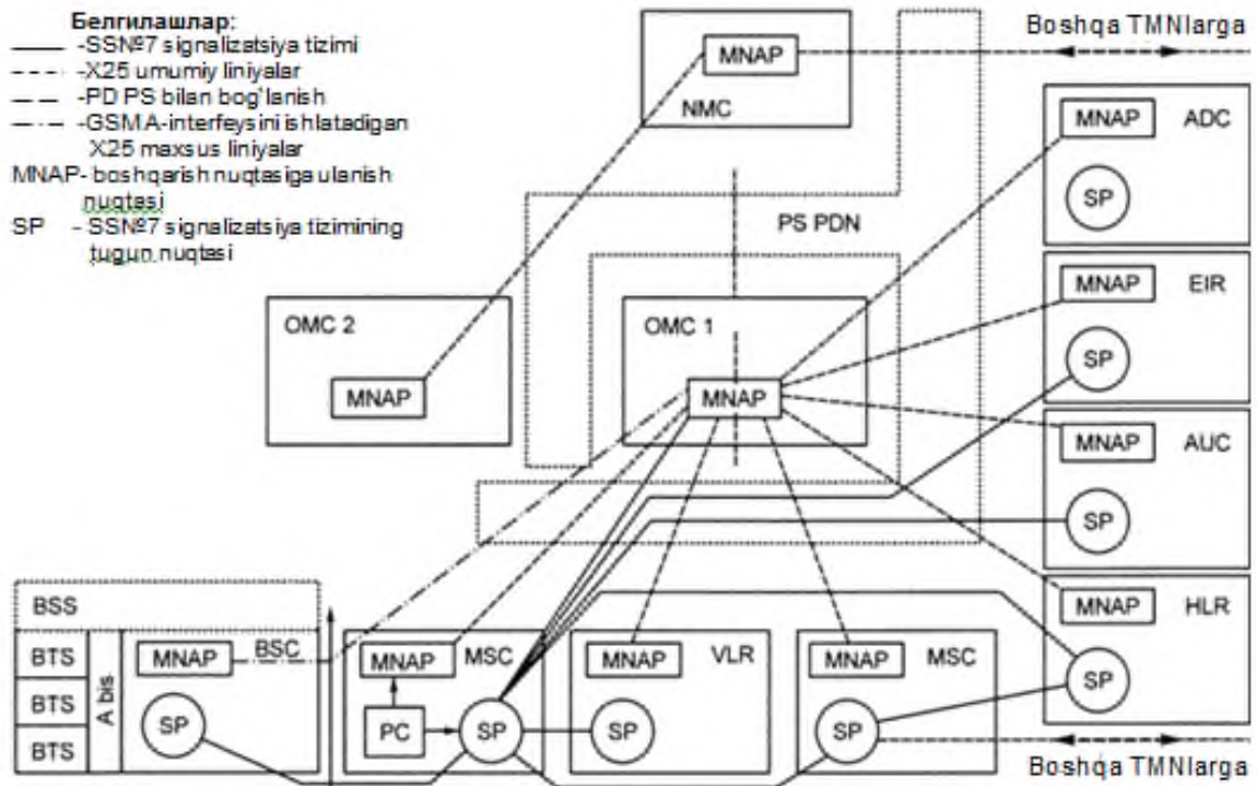
5.2- rasm. GSM TMN interfeyslari
