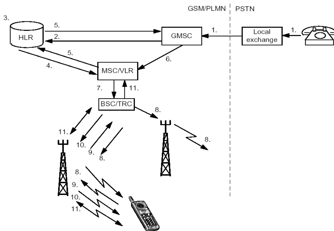
2.20- rasm. Kirish chaqiruvi (PSTN- MS)
