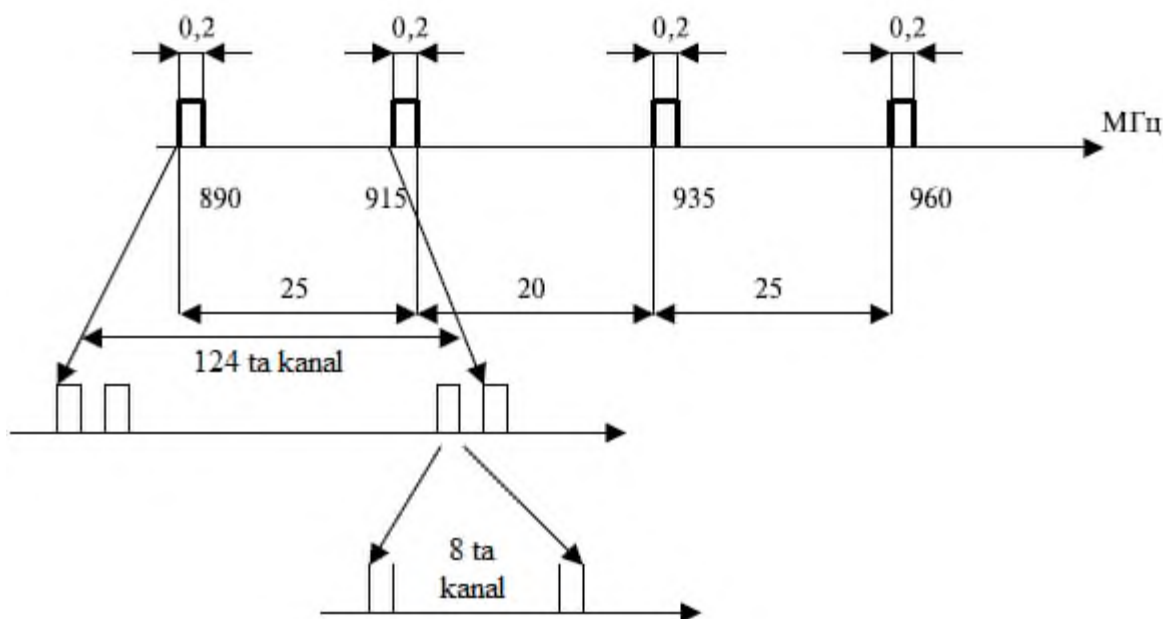
3.12- rasm.GSM tizimida kanallarning hosil bo'lishi
