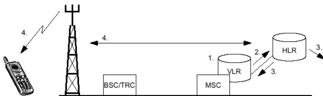
2.17- rasm. MSC/VLR xizmat ko‘rsatish zonasiga kirishda joylashish o‘rnini yangilash
