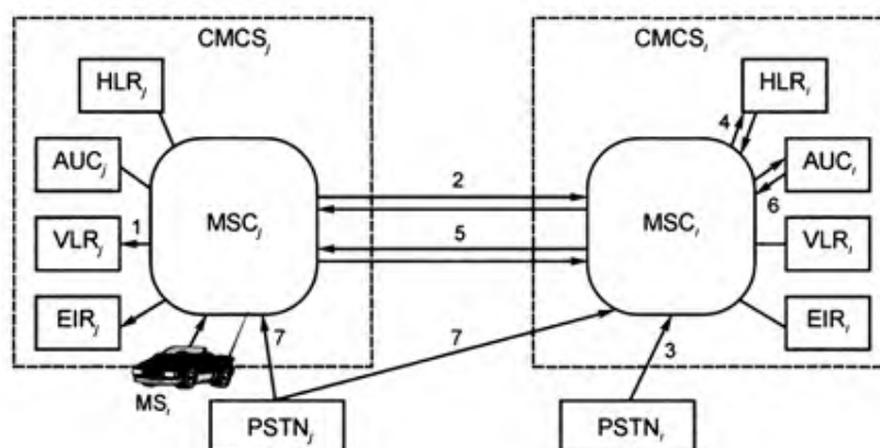
2.3- rasm. Roumingda GSM tarmoqlarining asosiy o'zaro ta'sirlashish protseduralari
