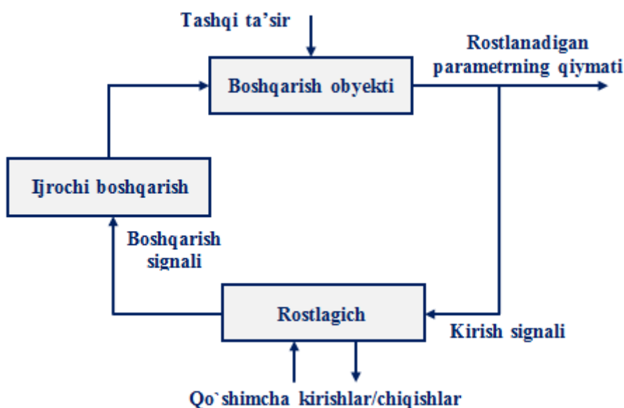
6.2- rasm. GSM-boshqarishning prinsipial sxemasi
